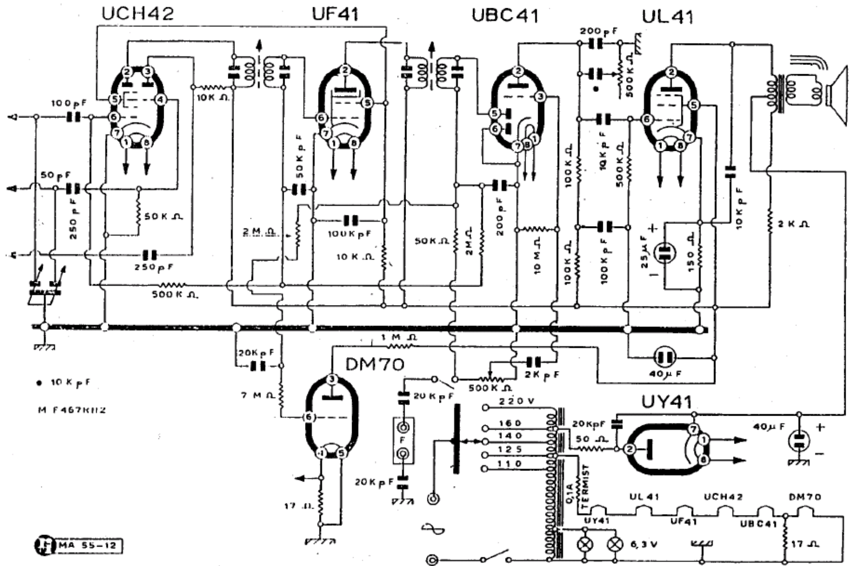
ELECTA RADIO - Mod. 524
